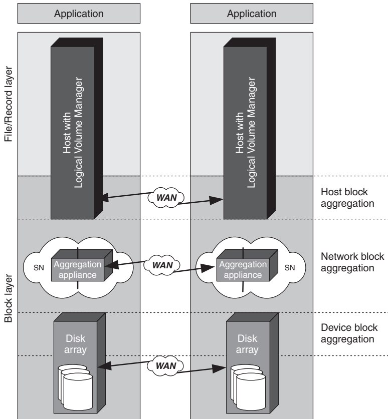
Figure 12.15 Data replication between two locations by means of WAN technology can take place at host level between volume managers, at network level between specialised devices, or at storage device level between disk arrays.
