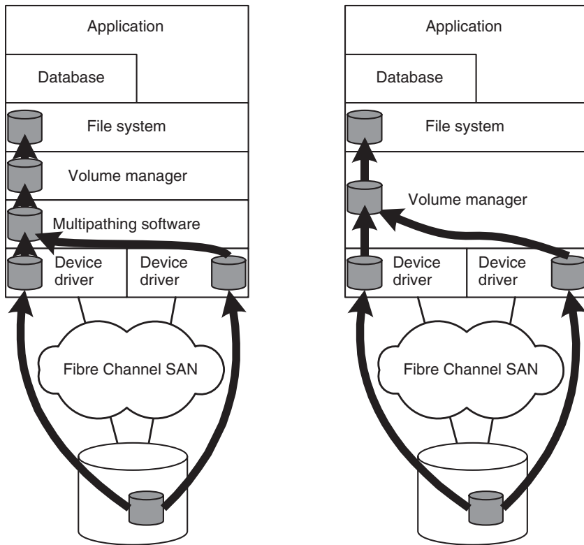
Figure 6.14 Solution: Multipathing software brings the multiply recognised disks back together. Multipathing software can be realised at various points in the operating system.
