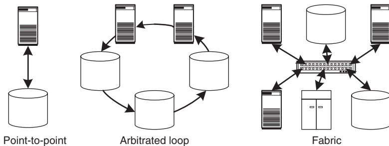
Figure 3.9 The fabric topology is the most flexible and scalable Fibre Channel topology.
