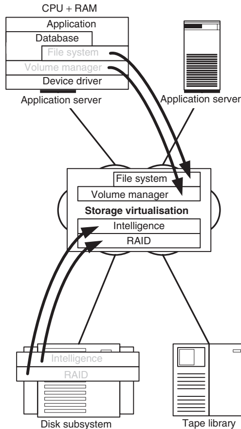
Figure 5.1 Storage virtualisation in the storage network moves virtualisation functions from servers and storage devices into the storage network. This creates a new virtualisation entity which, as a result of its central position in the storage network, spans all servers and storage systems and can thus centrally manage all available storage resources.
