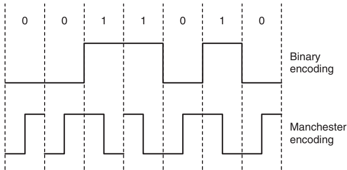
Figure 3.11 In Manchester encoding at least one signal change takes place for every bit transmitted.
