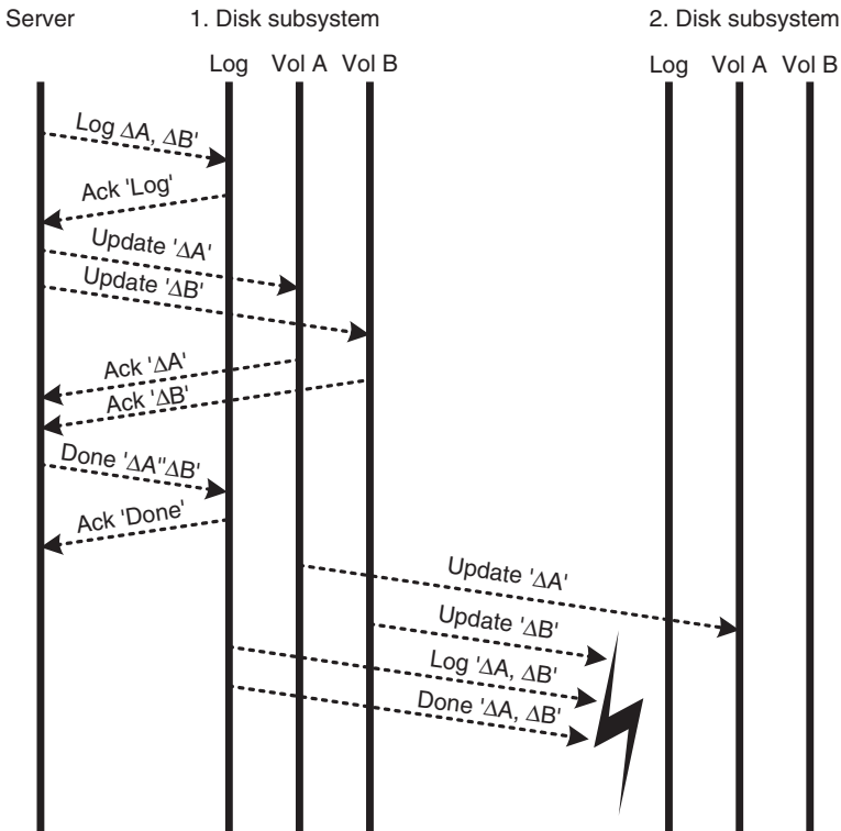
Figure 2.25 The consistency mechanism of databases and file systems records changes to data in a log, requiring adherence to a very specific sequence for writing in the log and the data. With asynchronous remote mirroring this sequence can be changed so that the start-up of an application will fail if a copy is used. The write-order consistency for asynchronous remote mirroring ensures that the copy is changed in the same sequence as the original on all the disks.
