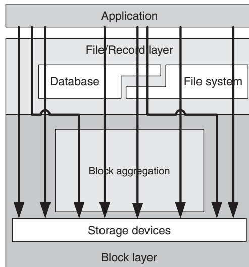
Figure 12.6 In the SNIA Shared Storage Model, applications can access the storage devices via eight possible access paths.
