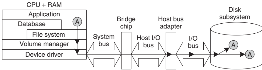
Figure 5.3 Virtualisation in the disk subsystem frees up server and storage network.
