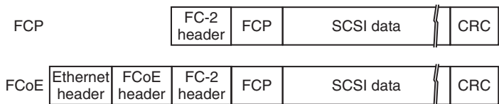
Figure 3.49 FCoE encapsulates Fibre Channel Frames 1:1 into Ethernet Frames.
