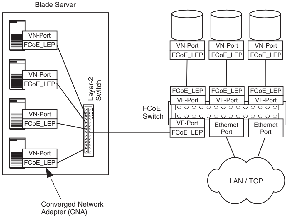
Figure 3.56 The internal layer-2 Ethernet switch connects the FCoE ports of the internal blade server modules and the ports of the external FCoE switch. The FCoE switch forwards incoming FCoE frames to the storage devices. The blade server modules use the same path to connect to the LAN.
