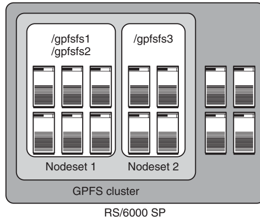
Figure 4.13 GPFS introduces the node sets as an additional management unit. GPFS file systems are visible to all nodes of a node set.
