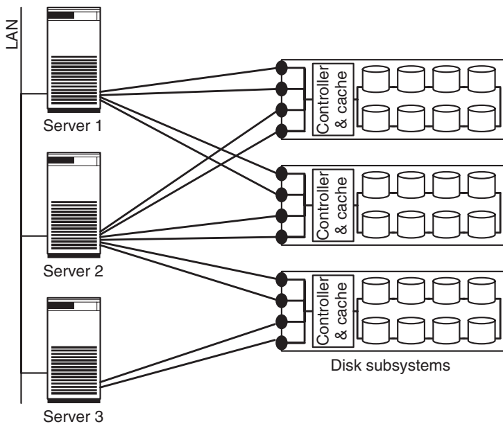
Figure 6.11 Redundant SCSI cable between server and disk subsystem protects against the failure of a SCSI cable, a SCSI host bus adapter or a connection port in the disk subsystem.
