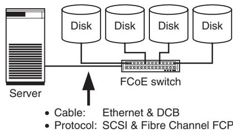
Figure 3.54 FCoE still uses Fibre Channel FCP for sending data via the SCSI protocol. However, FCoE uses Ethernet as transmission technology and not Fibre Channel.
